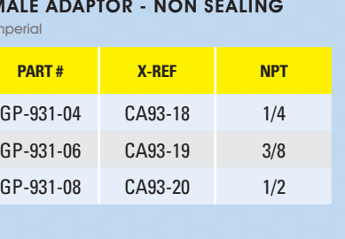
STYLE GP-931 MALE ADAPTOR - NON SEALING
