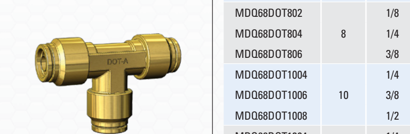
STYLE DQ64DOT / MDQ64DOT UNION TEE
