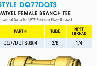
STYLE DQ77DOTS SWIVEL FEMALE BRANCH TEE
