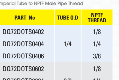
STYLE DQ72DOTS SWIVEL MALE BRANCH TEE
