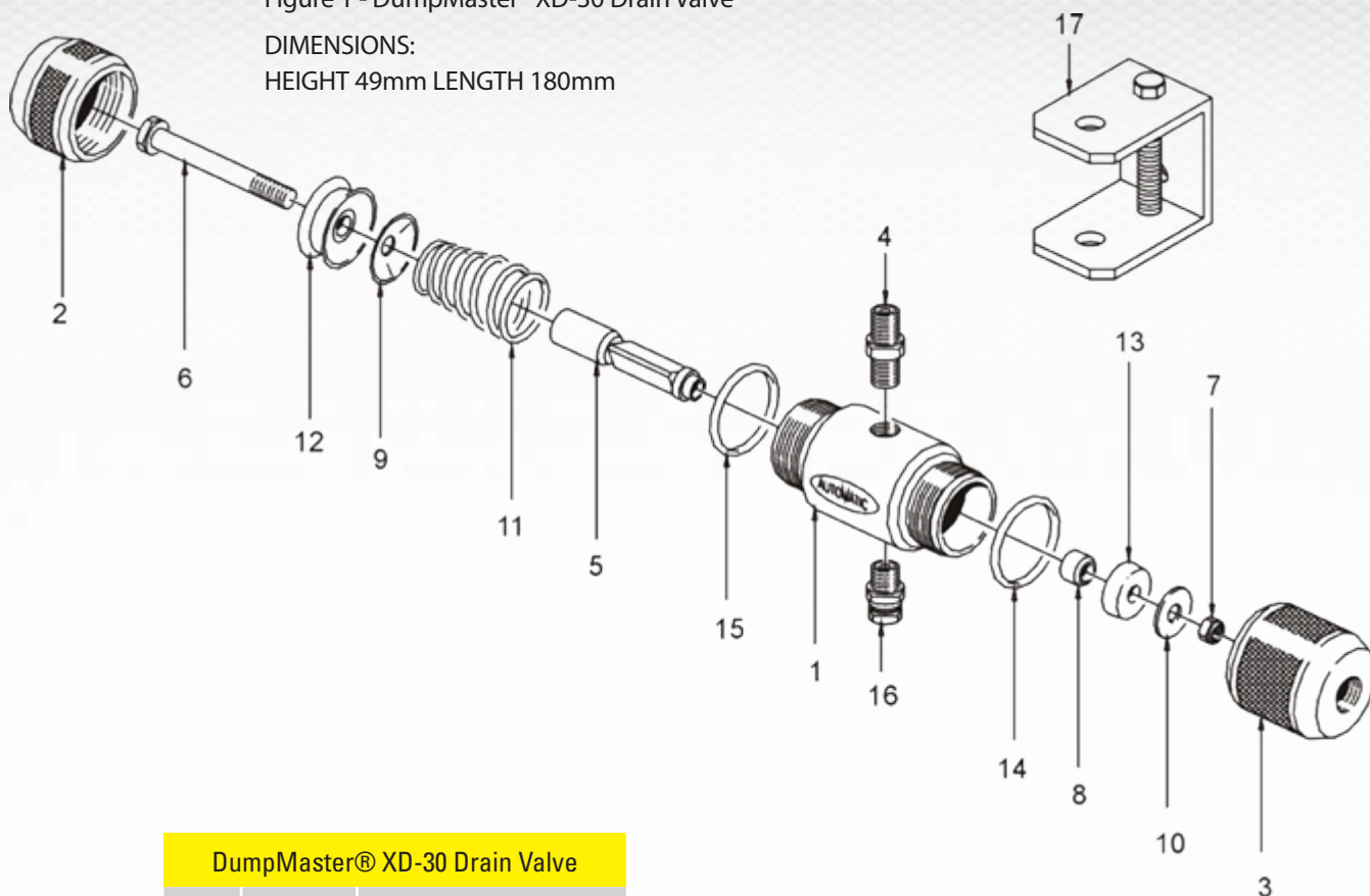
Figure 1 - DumpMaster® XD-30 Drain Valve
