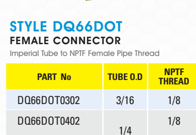
STYLE DQ66DOT FEMALE CONNECTOR
