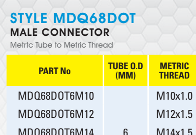
STYLE MDQ68DOT MALE CONNECTOR
