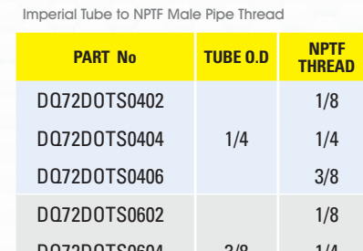
STYLE DQ72DOTS SWIVEL MALE BRANCH TEE
