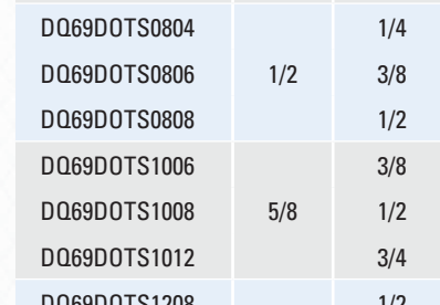
STYLE DQ70DOT FEMALE ELBOW
