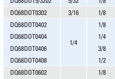
STYLE DQ68DOT MALE CONNECTOR
